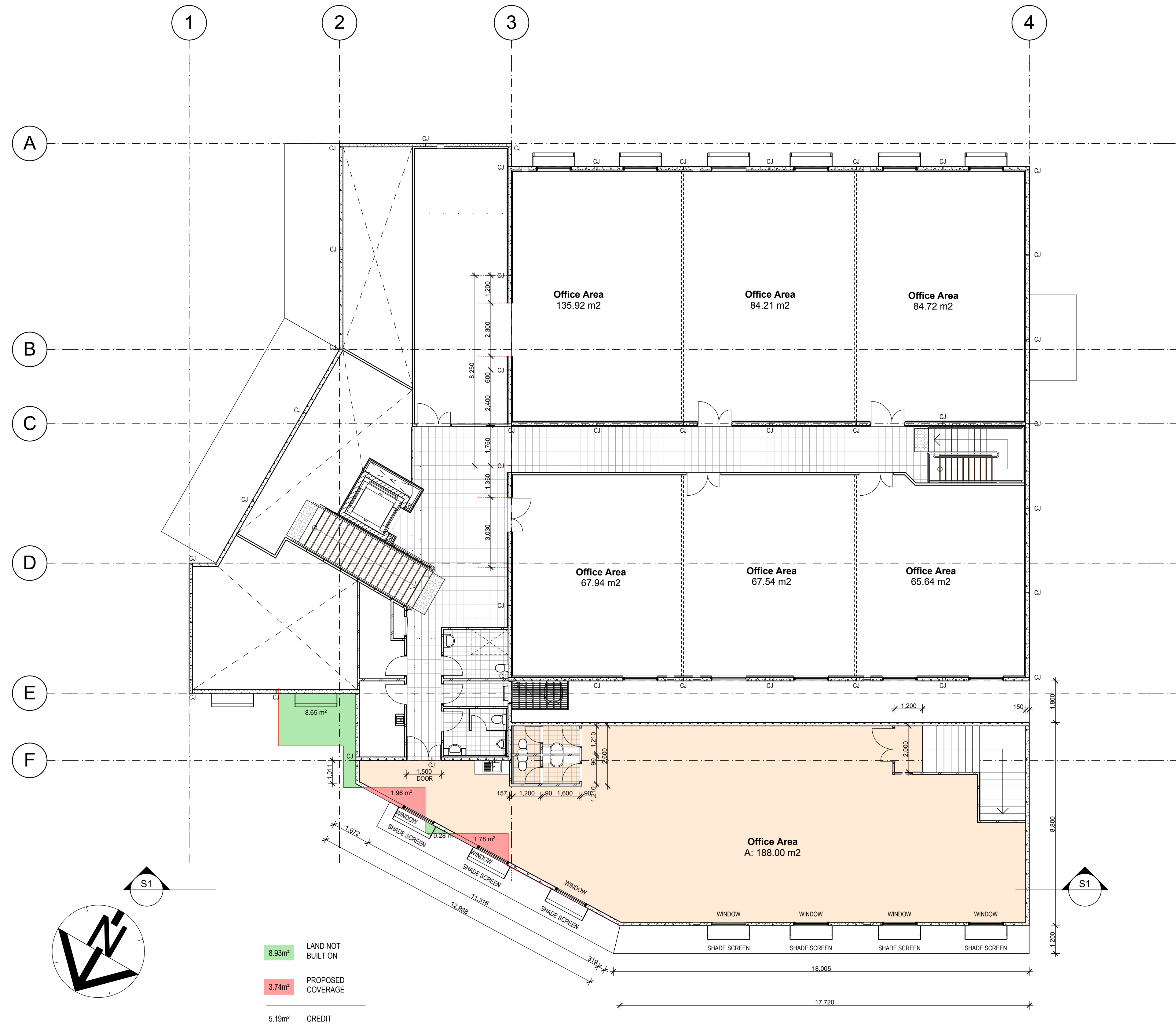
Karra Expansion (1st) Scale 1:100
